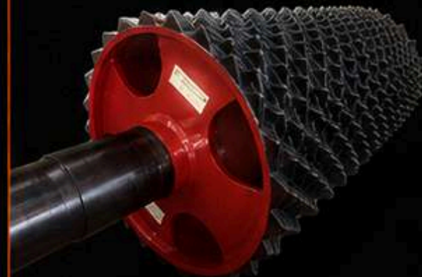
TOOTHED ROLLER
