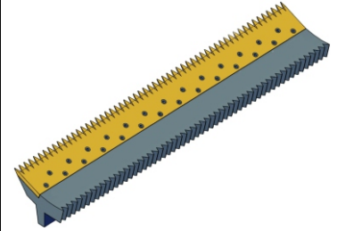
TRASH PLATE WITH REMOVABLE INSERT PLATE
